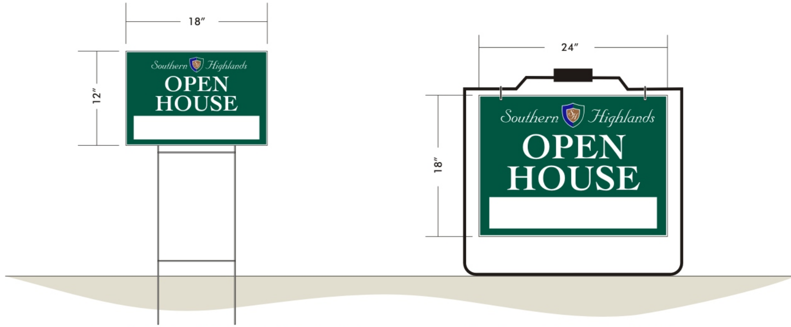
12"x18"x4mm D/F COROPLAST SIGN (VERTICAL FLUTES) W/ VINYL GRAPHICS INSTALLED ON WIRE-H-STAKE BOTH SIDES OF SIGN ARE IDENTICAL
